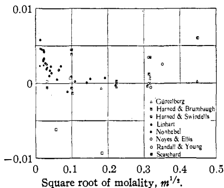
Fig. 4.—Difference between \log \gamma calculated from freezing point and electromotive force data.
