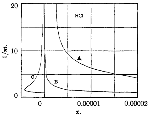
Fig. 3.— x -Function for hydrochloric acid.
